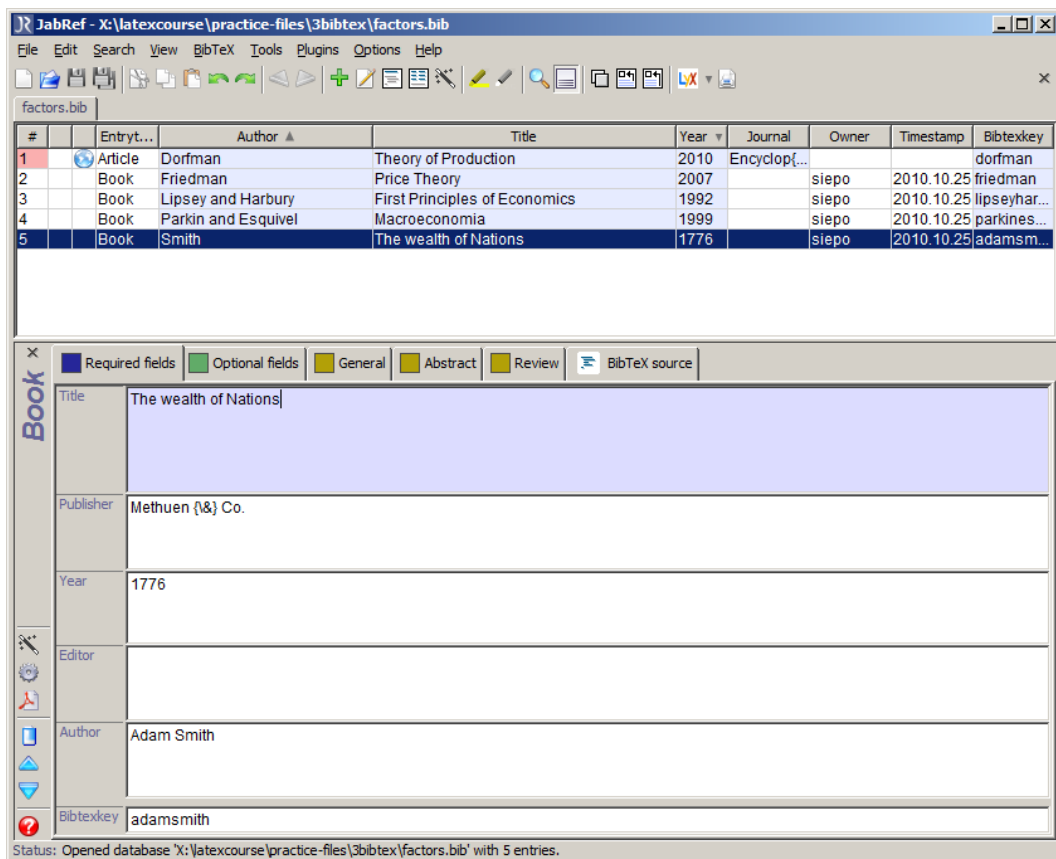
Figure C.1. JabRef BibTeX editor
